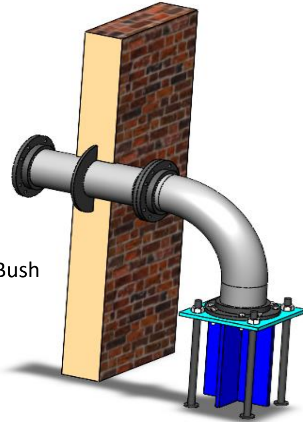
Antivortex Assembly with Elbow & Flange
