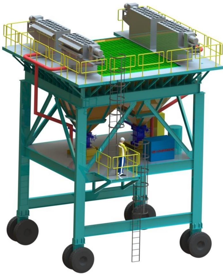
Mobile Hopper
