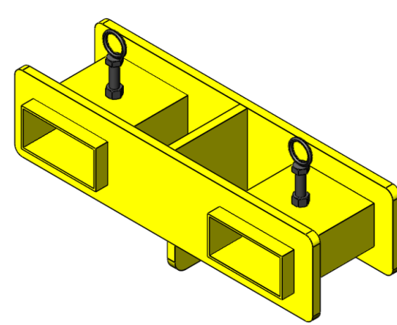
Forklift Cup
