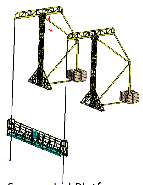
Suspended Platform
