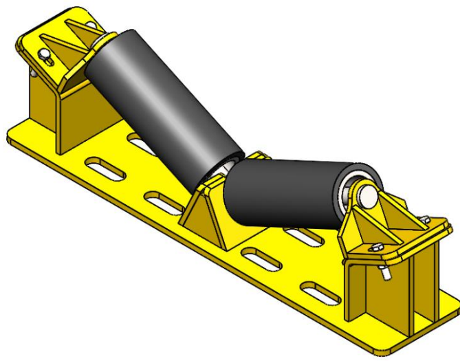
Horizontal Rigging Roller
