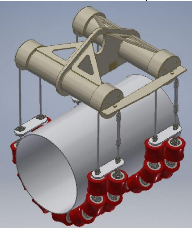
Pipe Rigging Cradle
