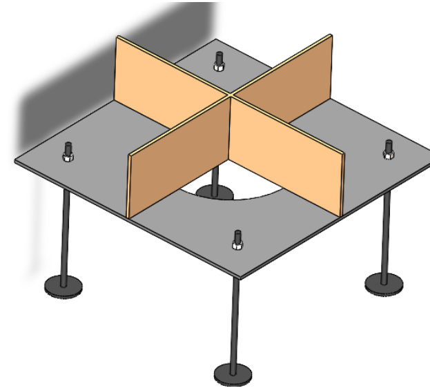
Antivortex Assembly Square
