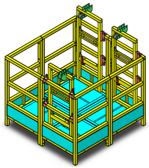
Suspended Platform
