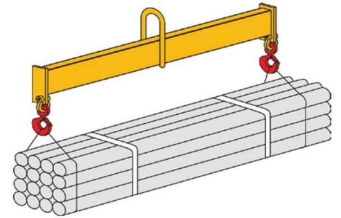
Lifting Beam
