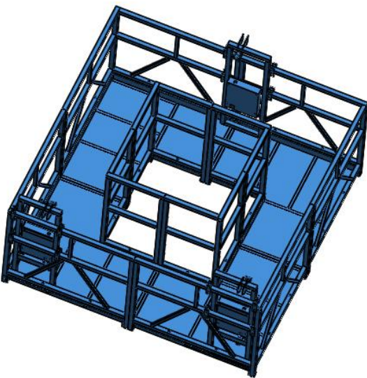
Suspended Platform
