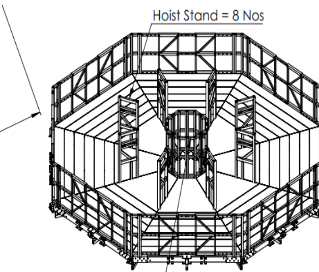
Suspended Platform
