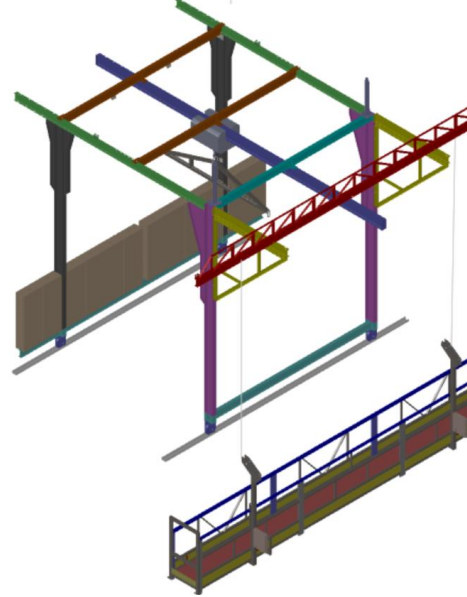
Suspended Platform
