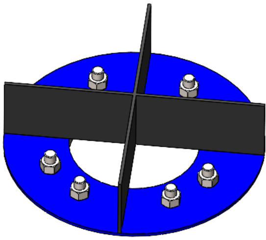
Antivortex Assembly Round
