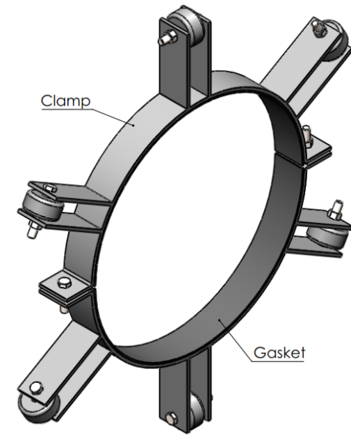
Casing Spacer
