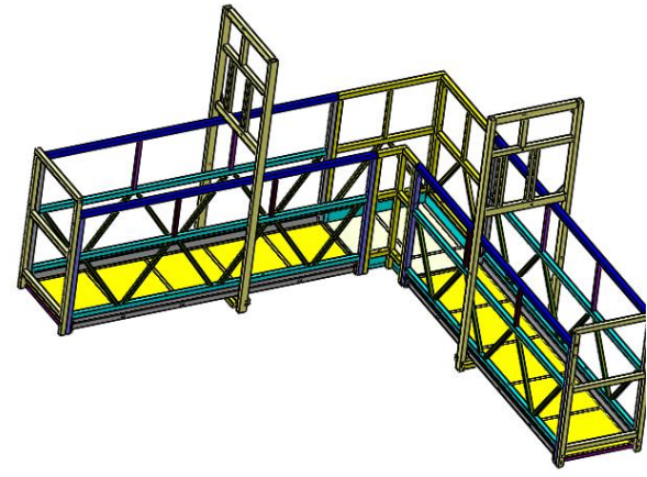
Suspended Platform
