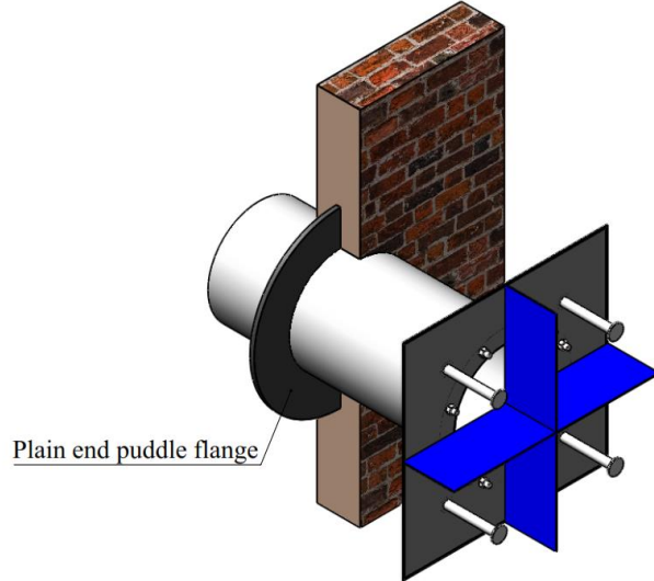
Puddle Flange
