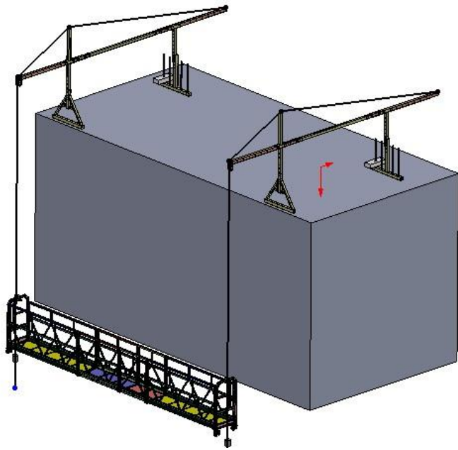
Suspended Platform
