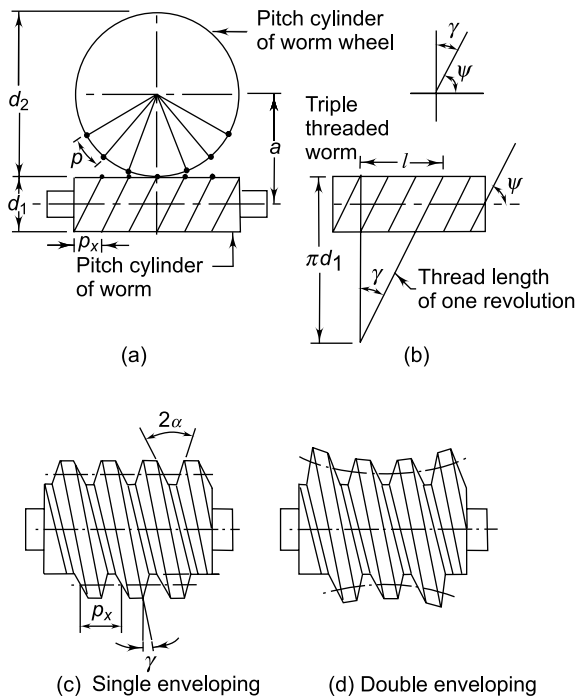
Fig. 20.1 Worm Gear Terminology
