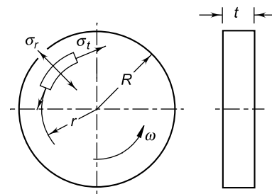
Fig. 21.6 Solid Disk Flywheel
