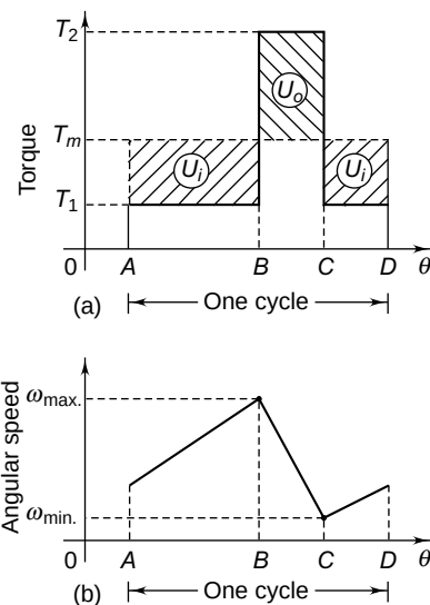
Fig. 21.4 (a) Torque Diagram (b) Speed Diagram
