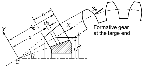
Fig. 19.17 Beam Strength of Bevel Gear Tooth
