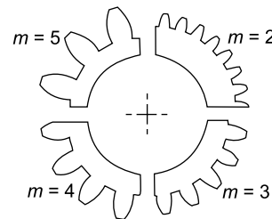
Fig. 17.12 Size of Gear Tooth for Various Modules
