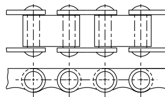
Fig. 14.4 Block Chain
