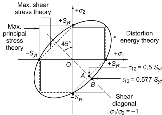
Fig. 4.37 Comparison of Theories of Failure
