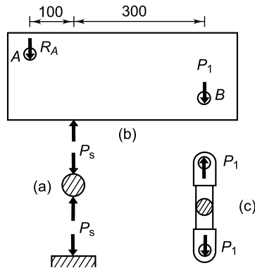
Fig. 4.58 Free-body Diagram of Forces
