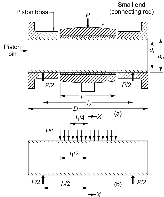
Fig. 25.9 Piston pin as beam
