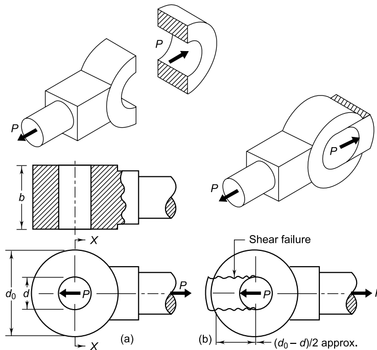
Fig. 4.23 (a) Tensile Failure of Eye (b) Shear Failure of Eye
