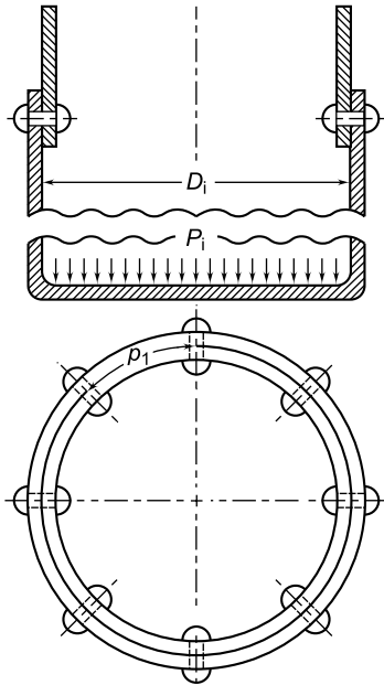
Fig. 8.65 Single-riveted Circumferential Lap Joint
