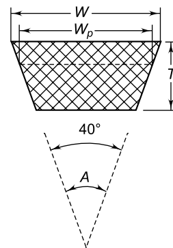
Fig. 13.23 Dimensions of V belt
