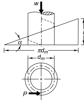
Fig. 6.5 Development of Thread
