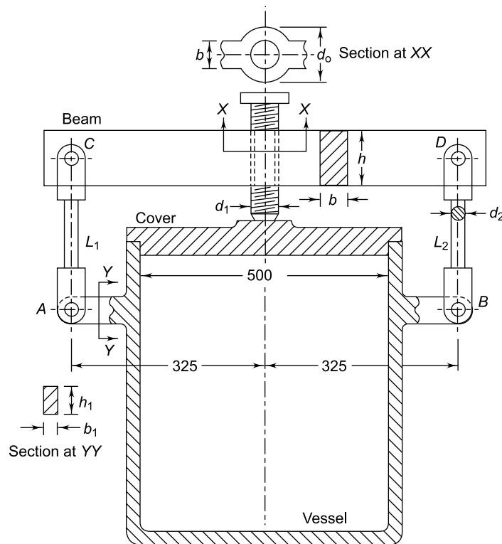
Fig 4.54 Pressure Vessel
