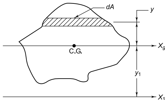
Fig. 4.6 Parallel-axis Theorem
