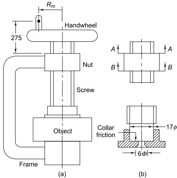
Fig. 6.15 C-clamp
