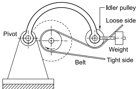
Fig. 13.26 Idler Pulley Mechanism
