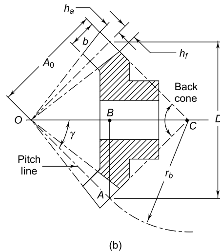
Fig. 19.6 Terminology of Bevel Gear
