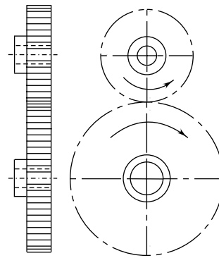
Fig. 17.1 Spur Gears
