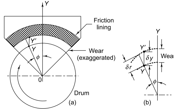
Fig. 12.11 Wear on Friction Lining
