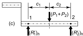
Fig. 25.27 Side crankshaft-bearing reactions
