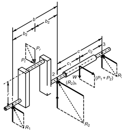
Fig. 25.24 Centre Crankshaft at Angle of Maximum Torque
