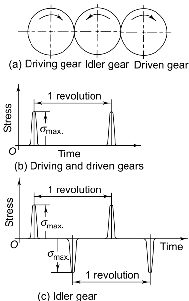
Fig. 17.41 Stress-time Diagram in Gear Teeth
