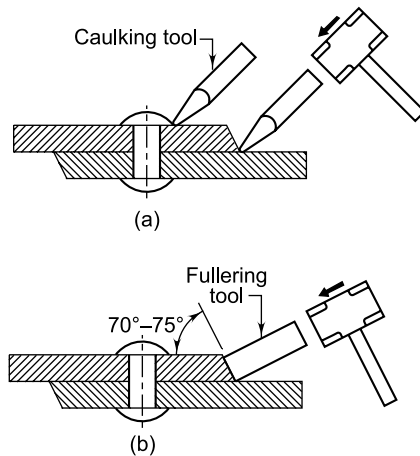
Fig. 8.58 Caulking and Fullering
