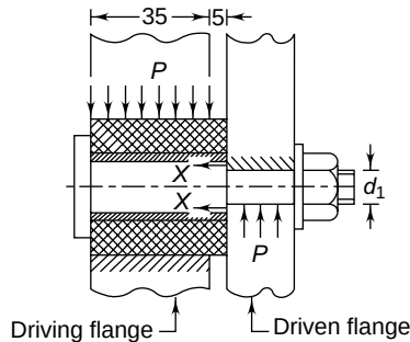
Fig. 9.43 Bearing Moment at Section XX
