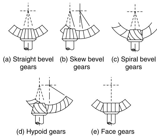
Fig. 19.5 Types of Bevel Gears
