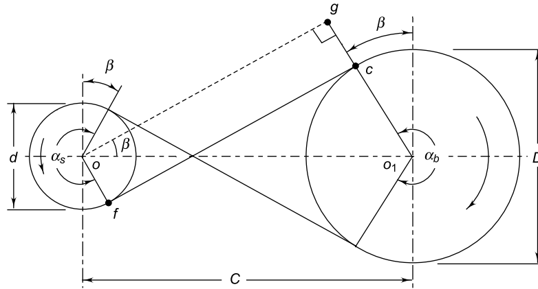
Fig. 13.6 Crossed Belt Drive
