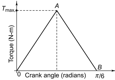
Fig. 21.17 Turning Moment Diagram
