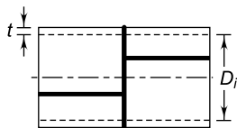
Fig. 22.16 Cylindrical Shell
