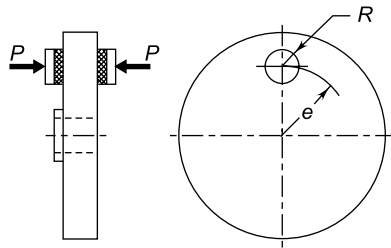
Fig. 12.28 Disk Brake with Circular Pad
