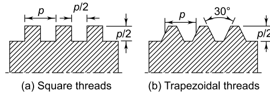
Fig. 6.1 Forms of Thread
