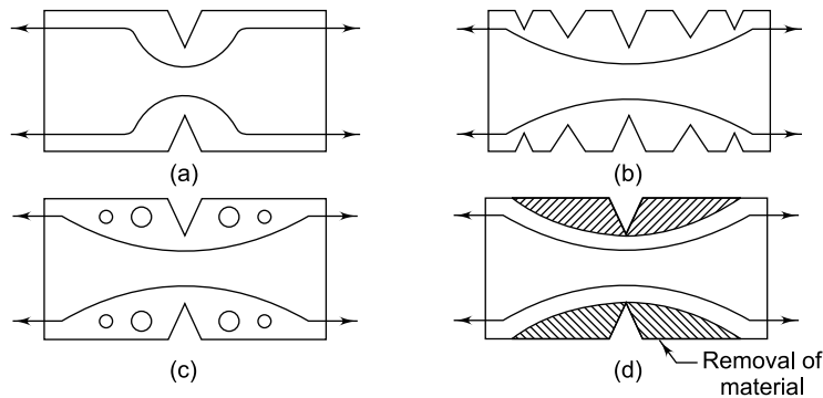
Fig. 5.9 Reduction of Stress Concentration due to V-notch: (a) Original Notch (b) Multiple Notches (c) Drilled Holes (d) Removal of Undesirable Material
