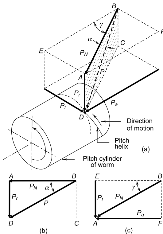
Fig. 20.6 Components of Normal Reaction
