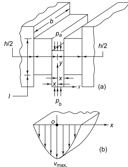
Fig. 16.12 Viscous flow through slot: (a) Rectangular slot (b) Velocity distribution
