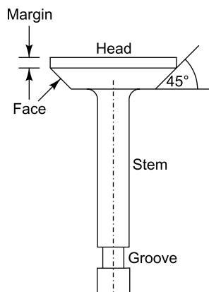
Fig. 25.32 Poppet Valve
