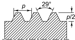
Fig. 6.2 Acme Threads
