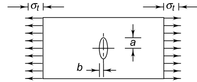
Fig. 5.7 Stress Concentration due to Elliptical Hole
