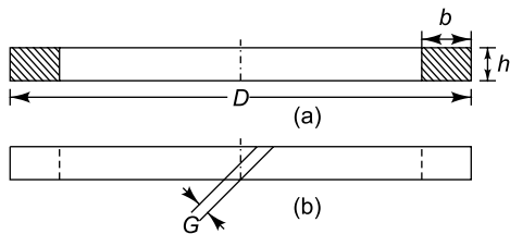
Fig. 25.6 Piston rings
