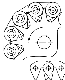
Fig. 14.16 Silent chain
