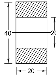
Fig. 4.60 Cross-section of Lever at Pin-C
