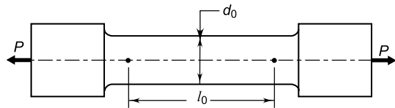
Fig. 2.1 Specimen of Tension-test
