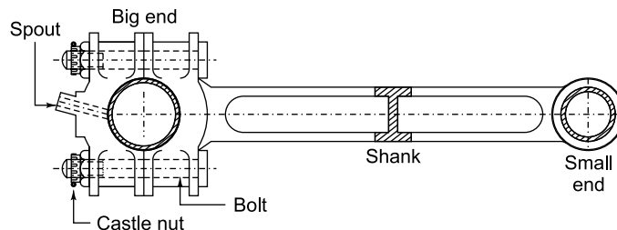
Fig. 25.12 Connecting Rod
