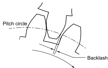
Fig. 17.19 Backlash
