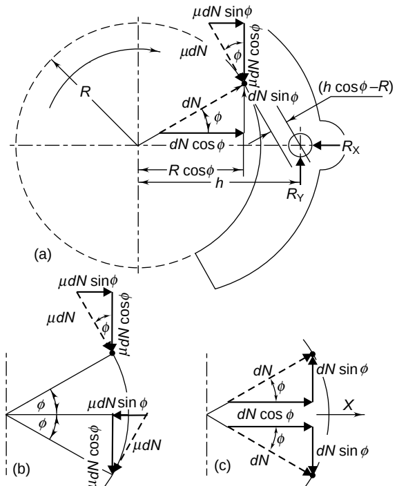
Fig. 12.15 Forces Acting on Shoe
