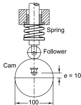
Fig. 10.21 Cam Mechanism
