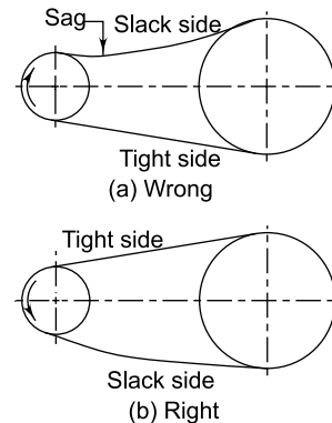
Fig. 14.12 Drive Arrangement
