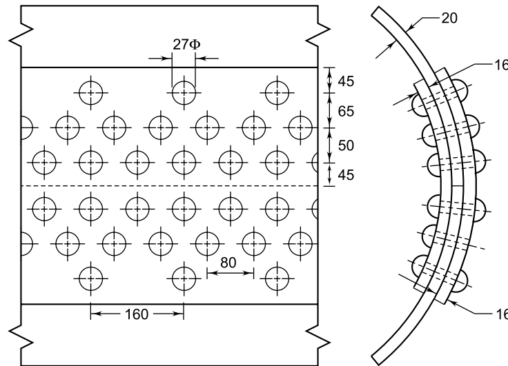
Fig. 8.63 Triple-riveted Double-strap Butt Joint with Equal Straps
