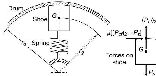
Fig. 11.16 Forces on Shoe
