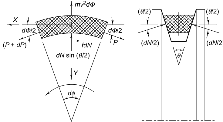
Fig. 13.8 Forces on V-belt
