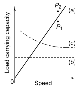
Fig. 16.34 Load Characteristics of Bearings: (a) Hydrodynamic Bearing (b) Hydrostatic Bearing (c) Rolling Contact Bearing
