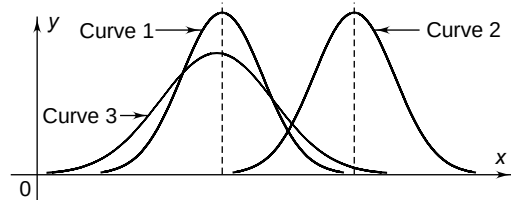
Fig. 24.3 Comparison of Central Tendencies
