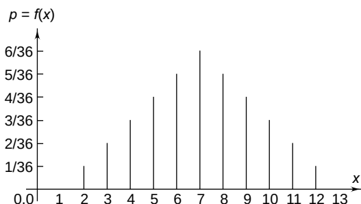
Fig. 24.8 Probability Distribution
