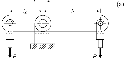
Fig. 4.42 Construction of Lever
