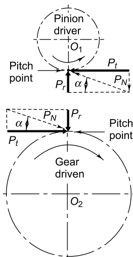
Fig. 17.21 Components of Tooth Force
