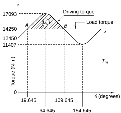
Fig. 21.8 Turning Moment Diagram
