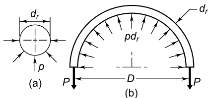
Fig. 23.5 Forces Acting on Wire Rope around Sheave
