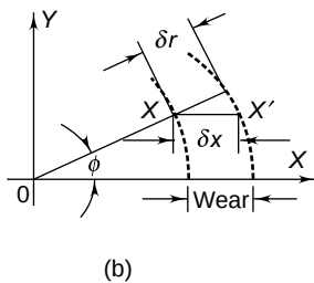
Fig. 12.14 Wear on Friction Lining
