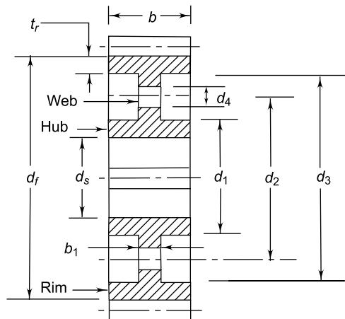
Fig. 17.34 Forged Gear
