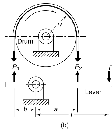
Fig. 12.23 Differential Band Brake: (a) Construction (b) Free-body Diagram
