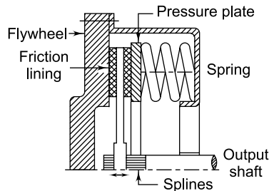
Fig. 10.19 Clutch Mechanism
