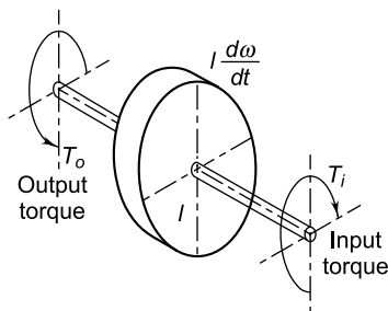
Fig. 21.3 Torque on Flywheel Shaft
