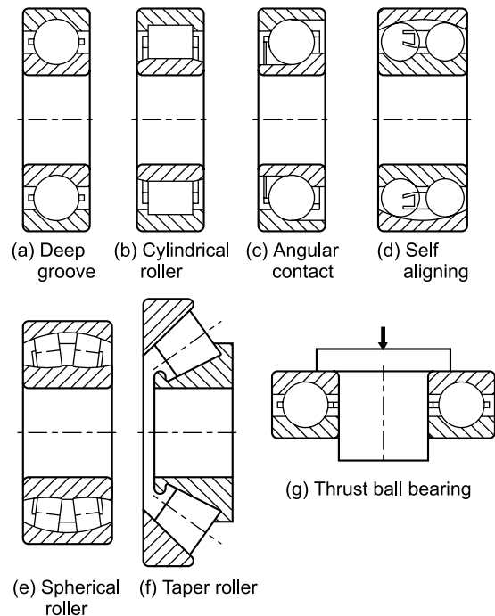
Fig. 15.3 Types of Rolling Contact Bearing
