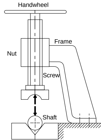
Fig. 6.14 Shaft Straightener
