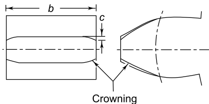
Fig. 17.13 Crowning of Gear Tooth
