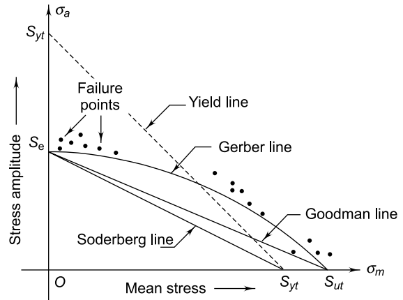
Fig. 5.39 Soderberg and Goodman Lines
