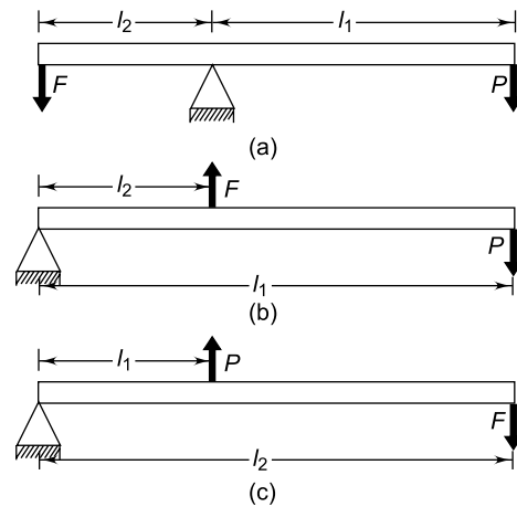
Fig. 4.43 Types of Lever
