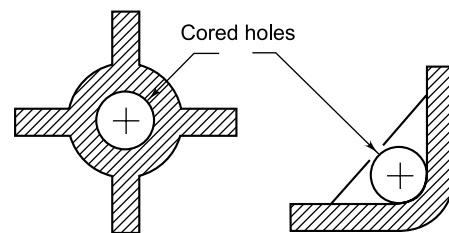
Fig. 3.6 Cored Holes
