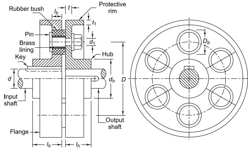
Fig. 9.39 Flexible Coupling
