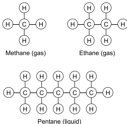
Fig. 2.8 Monomer Chains
