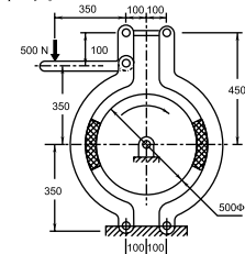
Fig. 12.6 Double Block Brake
