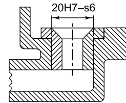
Fig. 3.26 Valve Seat
