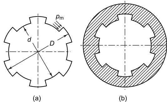
Fig. 9.27 Splines: (a) Shaft (b) Hub
