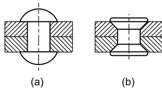
Fig. 8.47 (a) Shap Head Rivet (b) Counter Sunk Head Rivet
