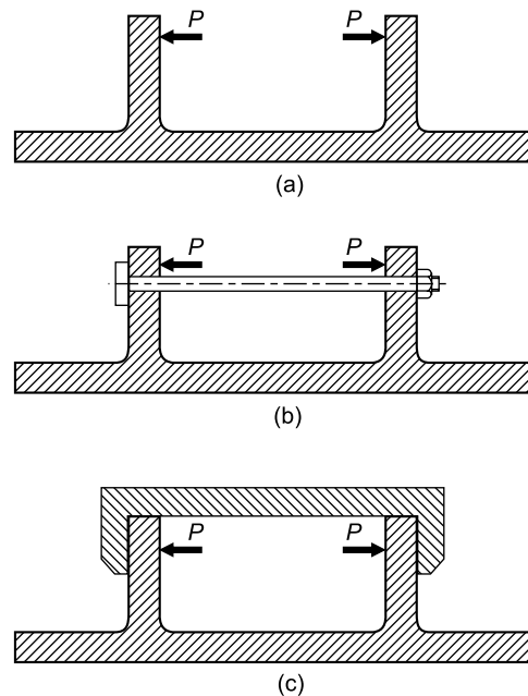
Fig. 3.2 (a) Original Component (b) Use of Tie-rod (c) Use of Bearing-cap
