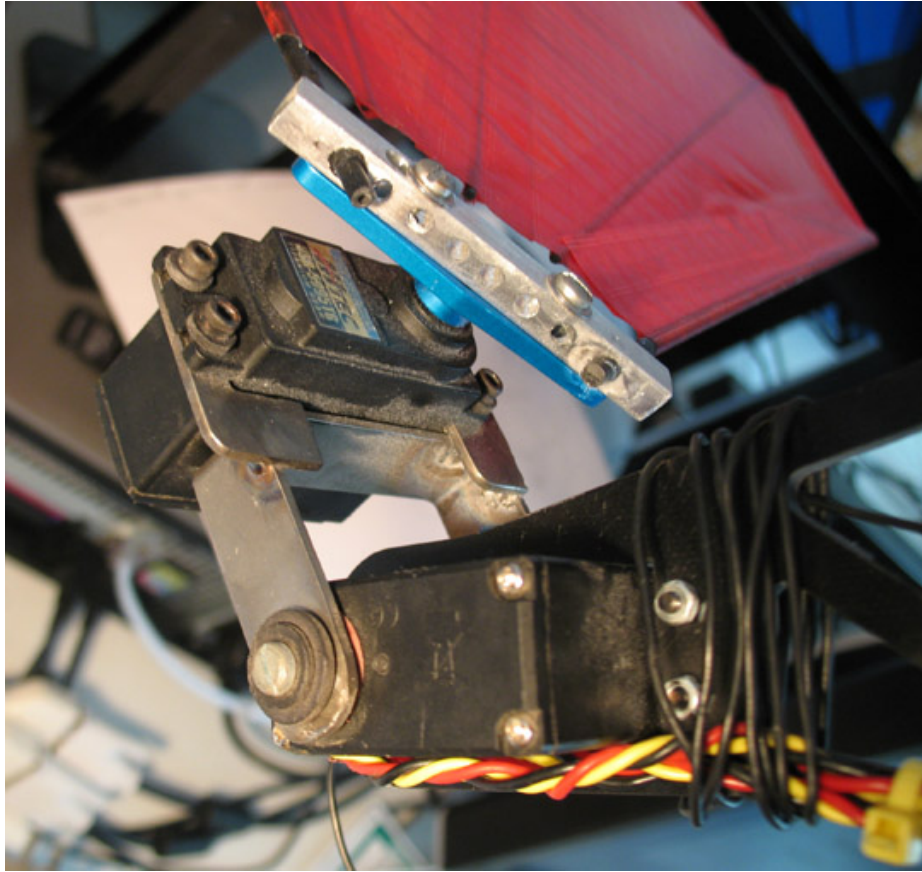
Figure 8-2: The tail section of the Phoenix. In contrast with the Kestrel the servos are directly joined in an effort to simplify the mechanism and save weight.
